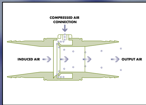
HOW THE RING JET AIR CONVEYORS WORKS
